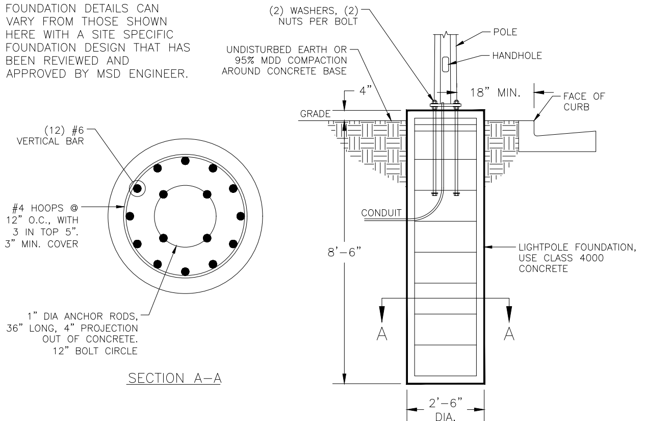
FOUNDATION DETAILS
